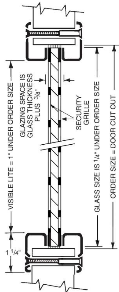
VLF-SG-S in Optional Stainless Steel Finish
